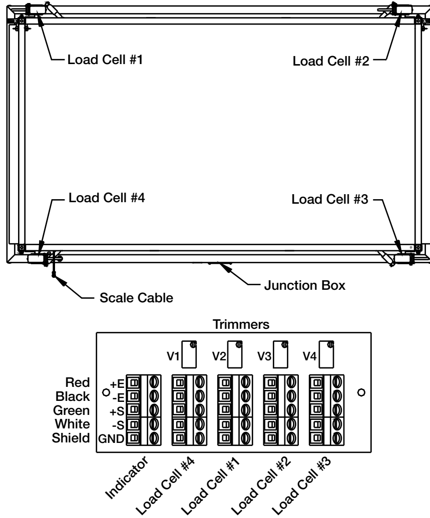
Figure 1. Updated wiring layout
